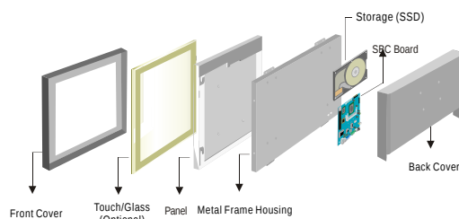
Mechanical design
